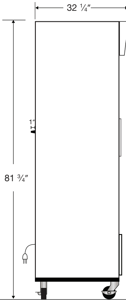
Side View
